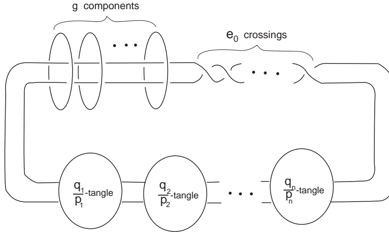
Figure 1: A generalised Montesinos link K(-g; e_0; \frac{q_1}{p_1}, \dots, \frac{q_n}{p_n}) .
