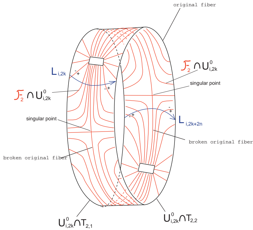
Figure 7: U_{i,2k}^0
