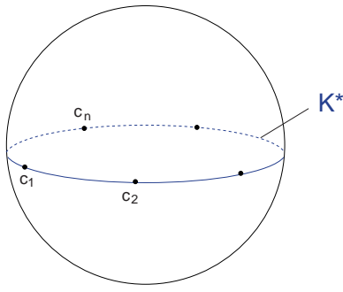
Figure 4: The orbifold S^2(p, \dots, p) with n cone points c_1, \dots, c_n , each with order p .
