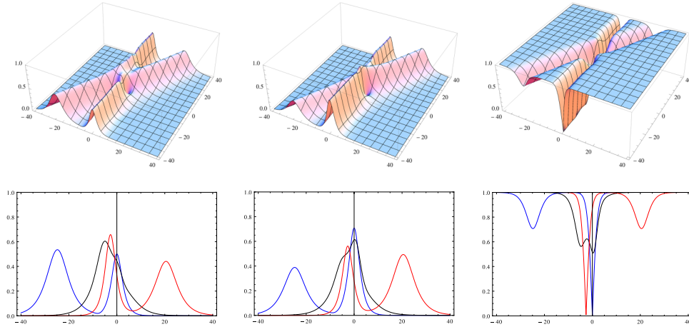
FIG. 1. A two-soliton solution of the 3-component defocusing VNL equation with NZBC obtained with discrete eigenvalues z_1 = i/2 and z_2 = (1+i)/4 , and norming constants \mathbf{c}_1 = (1, 1-i)^T and \mathbf{c}_2 = (i, 1+i/2)^T . The left, center, and right plots show the absolute value of each of the three components of \mathbf{q}(x, t) , respectively. The plots on the top show the value of the solution as a function of x and t . The plots on the bottom show the profile of each of the three components at t = -40 (blue), t = 0 (black), and t = 40 (red).
